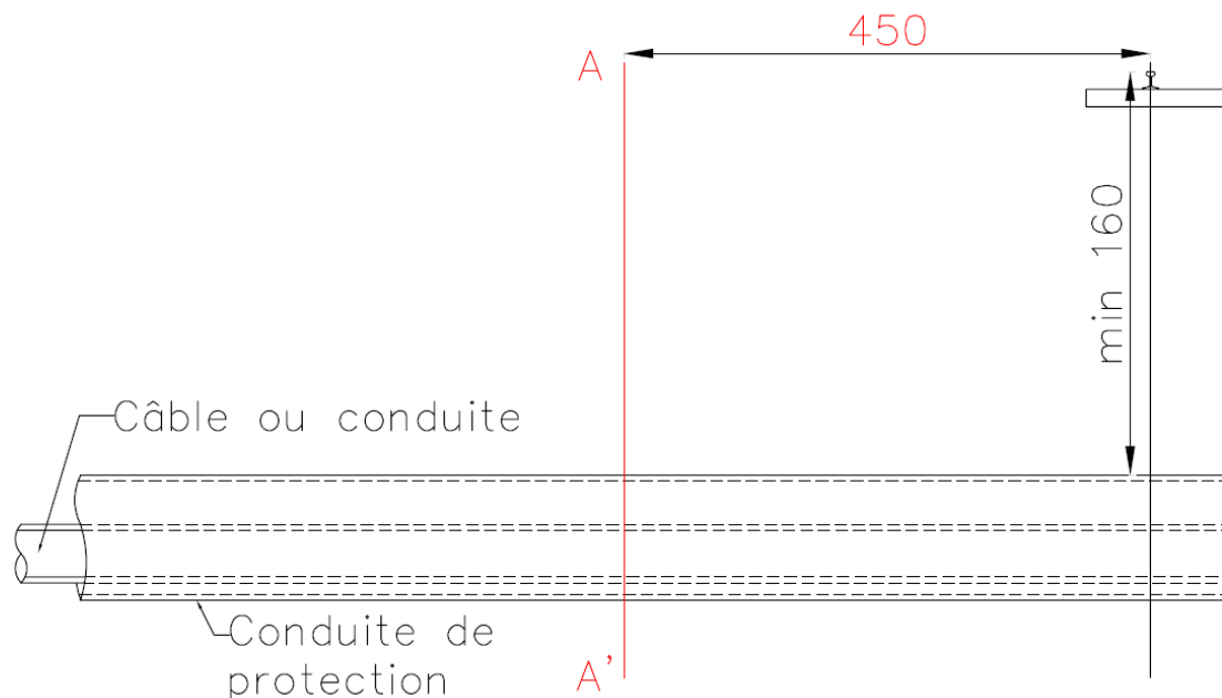
Figure 2.7 : Distance minimale
