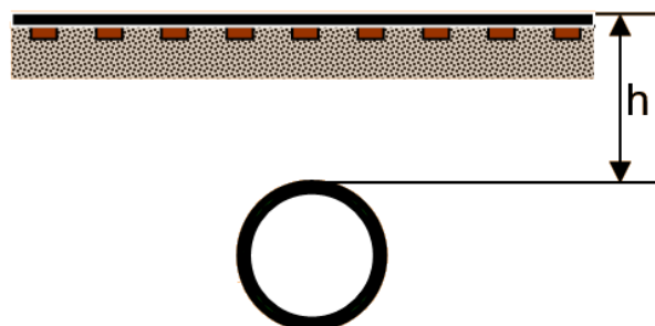
Figure 2.6 : Couverture minimale
